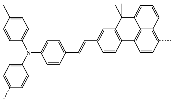
Formula 8
